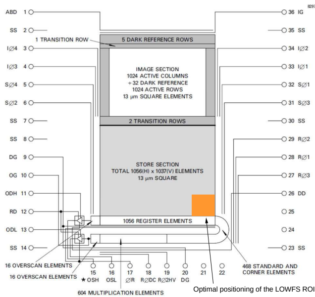
Figure 16: Position of the LOWFS ROI with respect to the CCD201-20 architecture (image adapted from [18]). For the CCD301, the store shield is not present.
