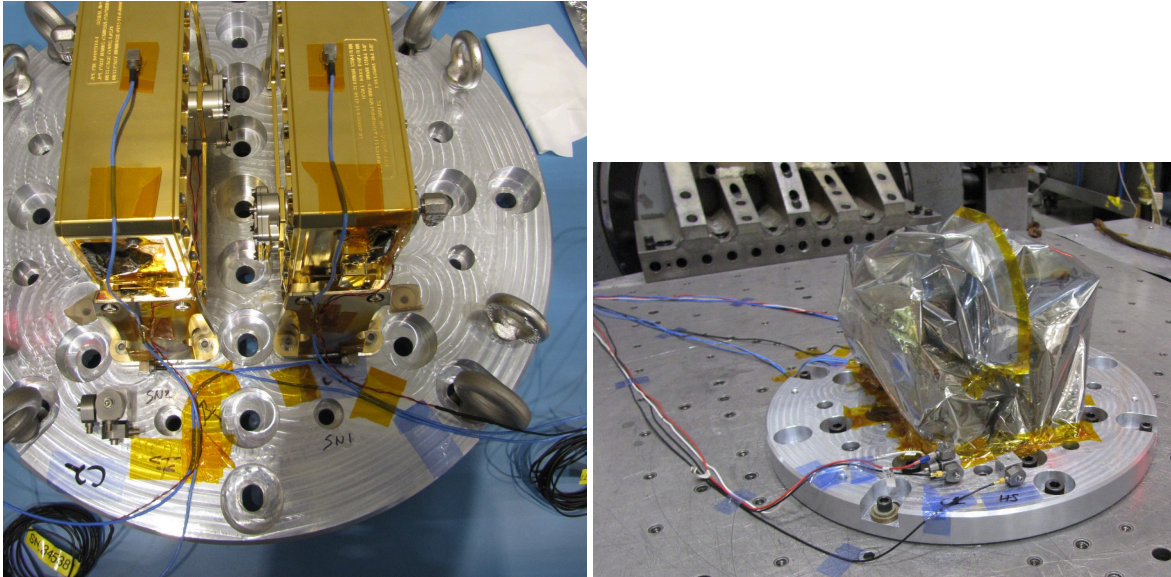
Figure 8: Setup of the CPEs for the vibration testing.
