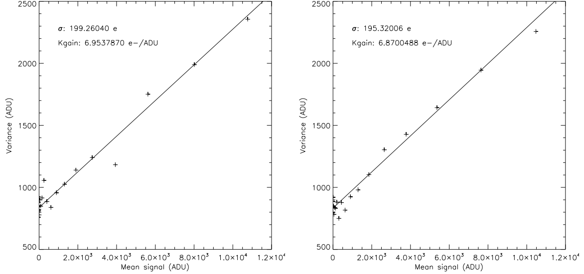
Figure 11: Photon Transfer Curve for both CPEs in TVAC. Left: SN1. Right: SN2.
