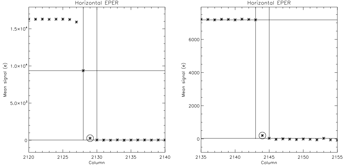
Figure 14: Horizontal EPER graphs for CTE measurements at unity gain. Left: SN1. Right: SN2.
