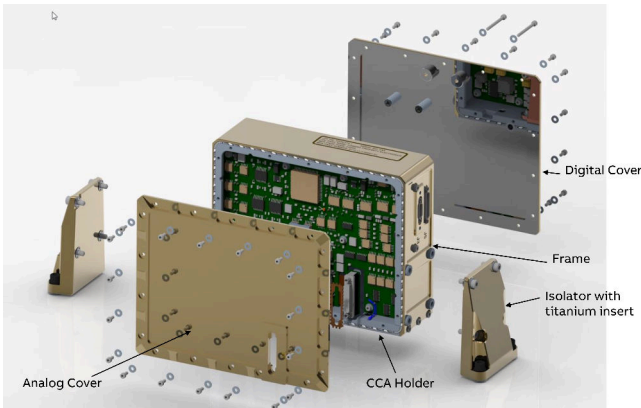
Figure 4: Exploded view of the CPE enclosure.
