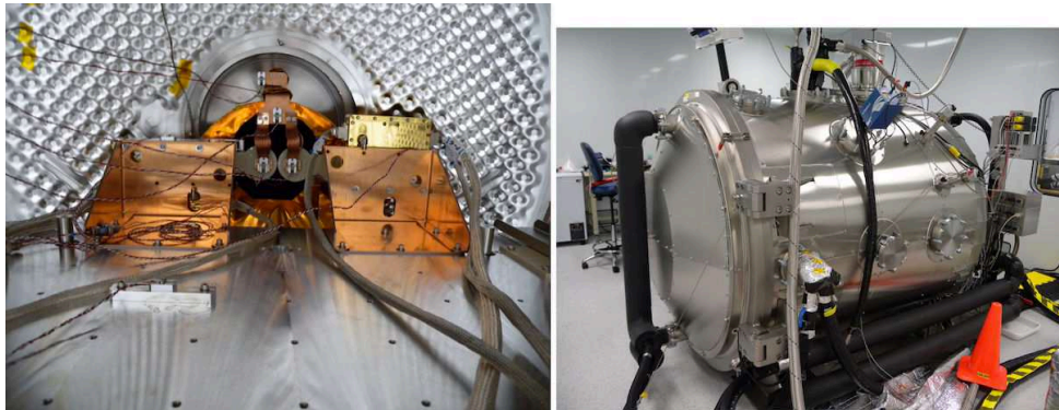
Figure 9: Left: Setup of the two CPEs in the TVAC at ABB, ready for the TVAC campaign. Right: Outside view of the TVAC in the clean room.
