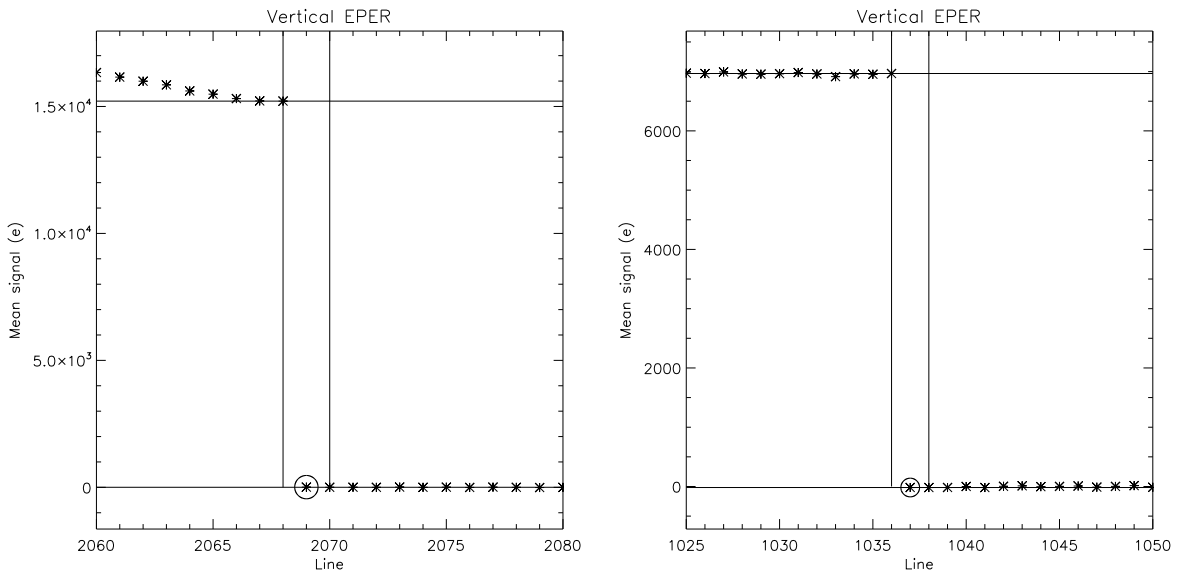
Figure 13: Vertical EPER graphs for CTE measurements. Left: SN1. Right: SN2.
