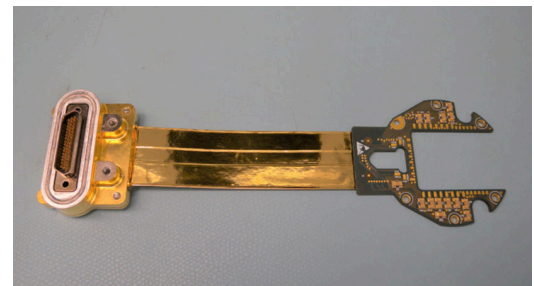
Figure 5: CPE's EMCCD headboard, showing the custom backshell and the gold tape on the flexible portion.
