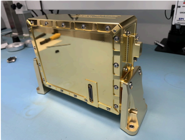
Figure 2: One of the flight CPEs on its PEEK buckets.
