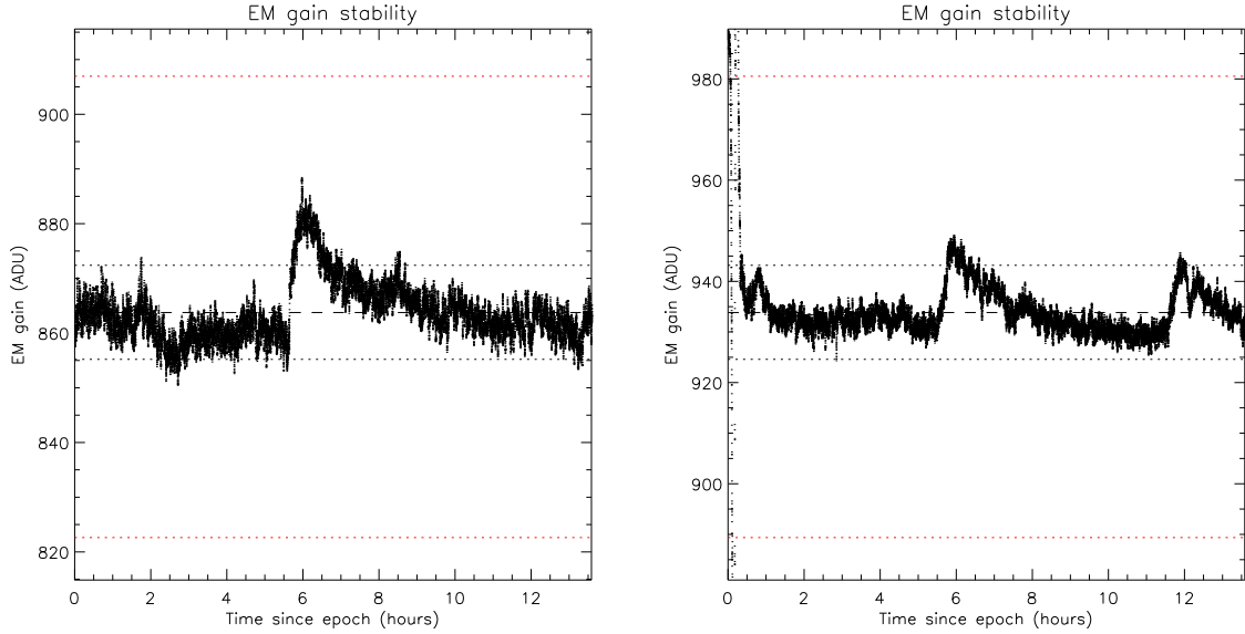
Figure 12: High gain stability. Left: SN1. Right: SN2. The red dotted lines represent a \pm 5\% variation, and the black dotted lines a \pm 1\% variation over the median.
