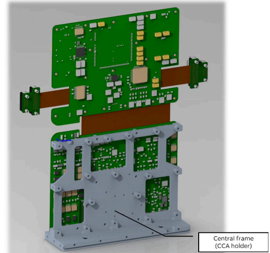
Figure 3: View of the flex-rigid PCB that composes the CPE electronics together with the center tray.
