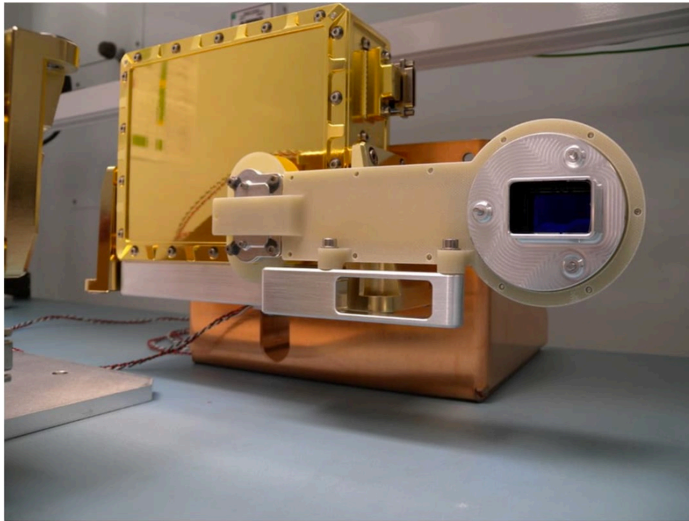
Figure 6: One of the flight CPEs (golden box) with a test EMCCD headboard attached, on a test jig (copper block) at ABB.
